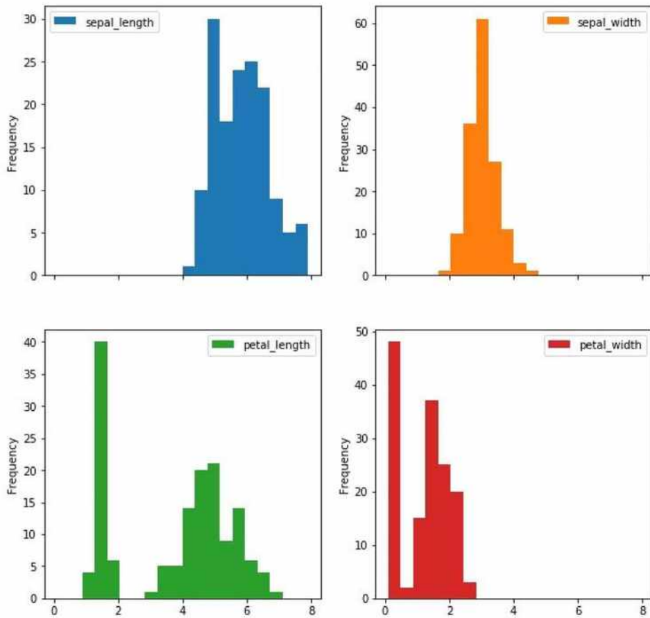
Figure 12: Multiple Histograms
