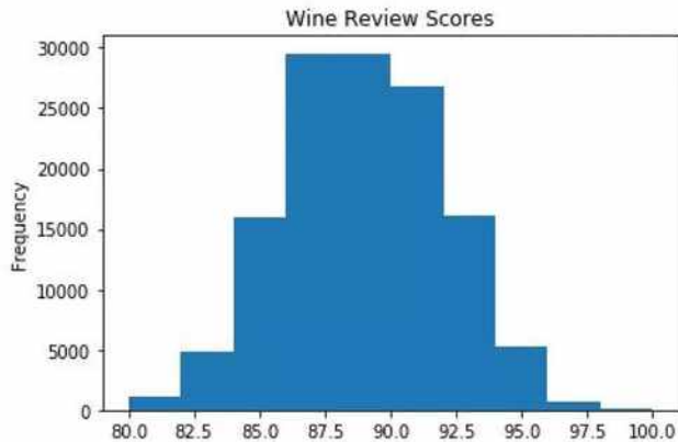
Figure: Histogram
